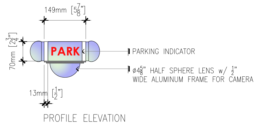
ALUMINUM PROFILE
