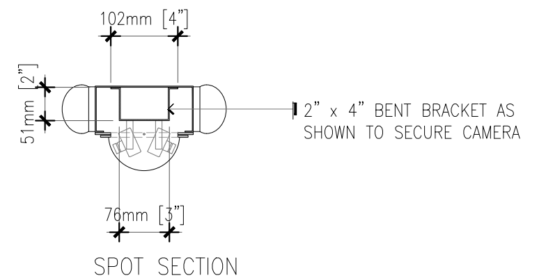
CAMERA BRACKET
